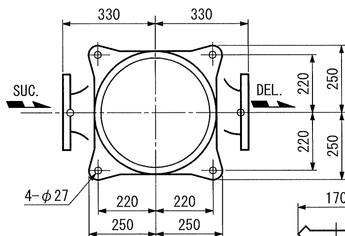
A-A ARROW VIEW
