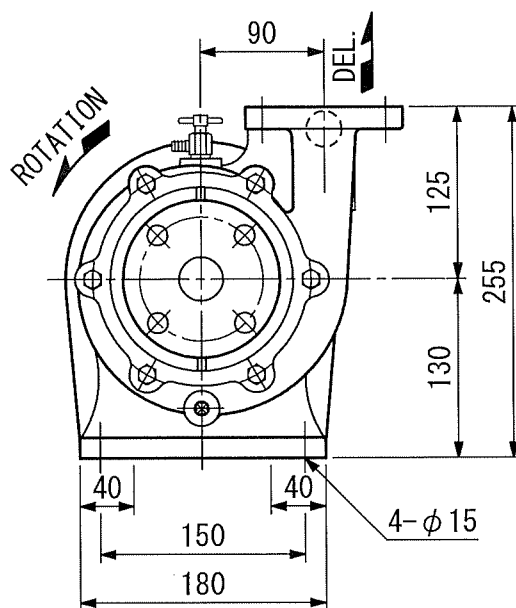
A-A ARROW VIEW
